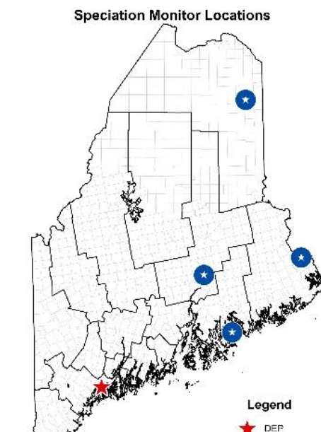
Figure 13: Speciation (IMPROVE)
